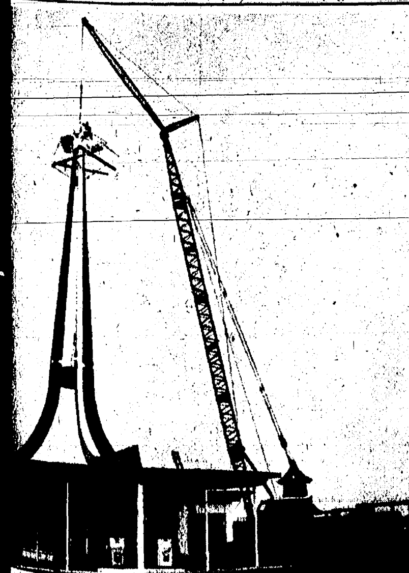
NEW SHELL SERVICE STATION—When the above photo was taken, the 110-foot boom was lowering the holder for the 10-foot revolving illuminated sign which will top the 90-foot tower at the Shell Service Station at I-94 and M-52. The top of the tower, which is constructed of laminated beams, is 90 feet from the ground. The 10-foot revolving sign on its 24-inch holder, adds 12 feet to the height bringing it to a total of 102 feet. It can be seen for miles in either direction on I-94. Burlin Brown is the general contractor on the construction of the new style of service station—the tower is expected to become a Chelsea area landmark. Two men were working atop the 90-foot tower when the photo was taken. They were on the catwalk, now enclosed only by an open railing. When completed, the catwalk will be enclosed on the outside, and will reflect the light of the revolving sign. The service station is to be operated by Harmon and Ann Arbor and is expected to open for business shortly. The new station is adjacent to the new Schumm restaurant which is under construction in preparation for opening in approximately six weeks.
